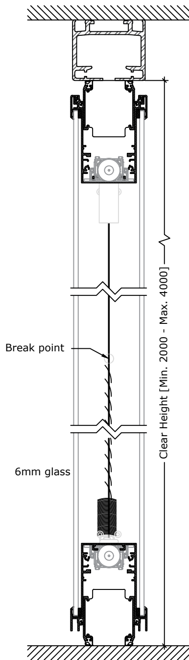
SECTION Scale 1:5
