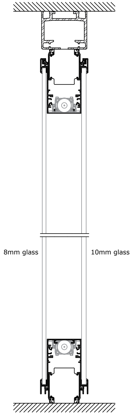
SECTION Scale 1:5
