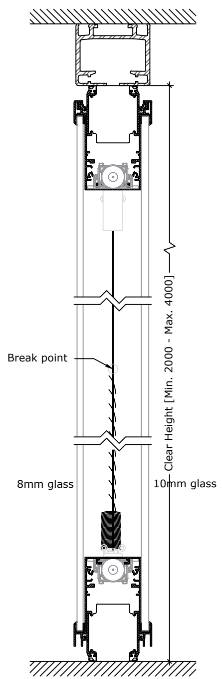
SECTION Scale 1:5
