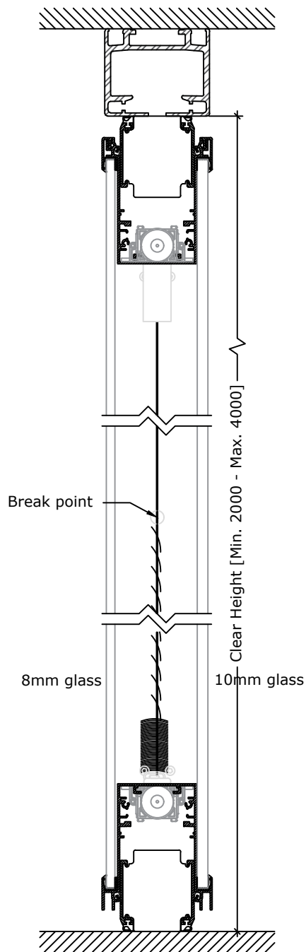
SECTION Scale 1:5
