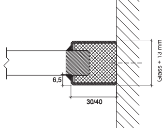
Wall connection
