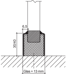
Floor connection
