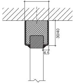
Ceiling connection
